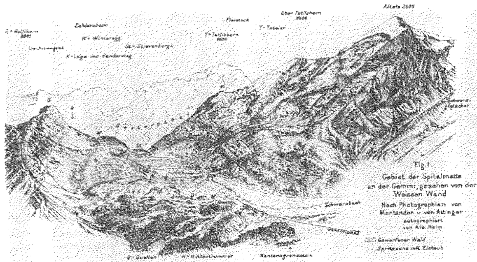
Fig.3.1 The ice avalanche from Altels. The curve-shaped line of rupture is visible immediately under the Altels summit (after Heim 1896).
