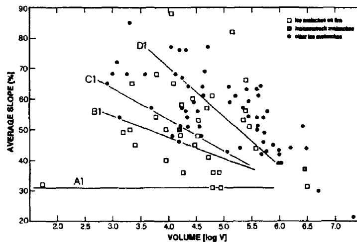
Fig.3.5 Average slopes (%) and volumes ( V in m^3 ) of ice avalanches (after Alean 1985).
