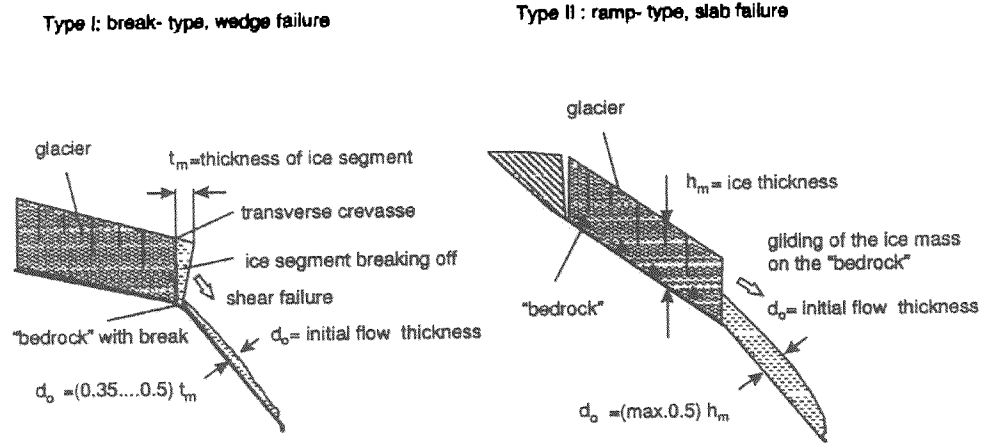
Fig.3.4 Types of starting zones (after Margreth and Funk 1998).
