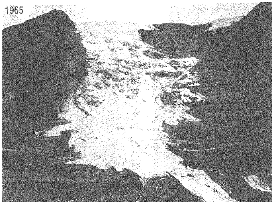
Fig.3.2 The ice avalanche from Allalingsletscher.
