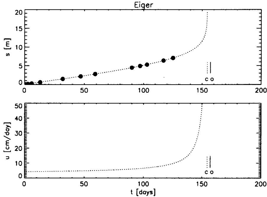
Fig.3.6 Upper panel: measured positions s_i (circles) and resulting hyperbolic function. Lower panel: velocity-time function. Day 0 corresponds to March 16, 1990. o: observed event (August 20, 1990) and c: calculated t_{\infty} (August 17, 1990).
