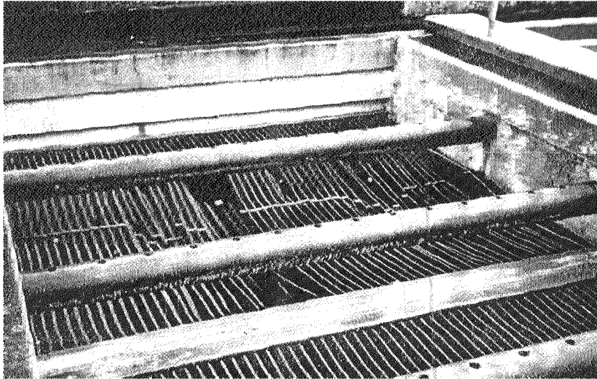
Figure 3-4 Plates damaged in clarifier in Limon, Costa Rica, 1991
