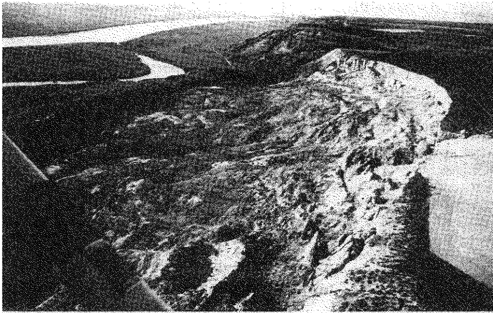
Figure 6. Aerial view of the Savage Island land- slide on the east shore of the Columbia River, Washington, 1981. This landslide was caused by irrigation water (photograph by Robert L. Schuster, U.S. Geological Survey).
