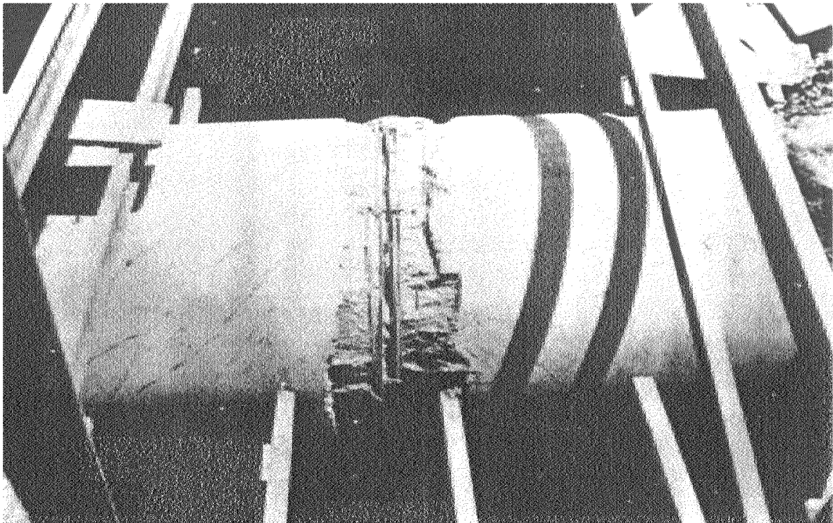
FIGURE 6-4 Crushing Failure In A 72"φ 'Lock Joint' Pipe, 1985 Michoacan Earthquake
