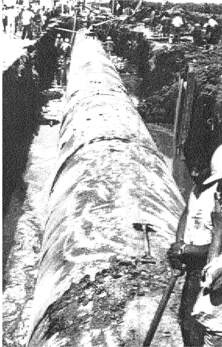
FIGURE 6-5 Joint Separation At 11 Points Close To A "T" Junction, 1985 Michoacan Earthquake
