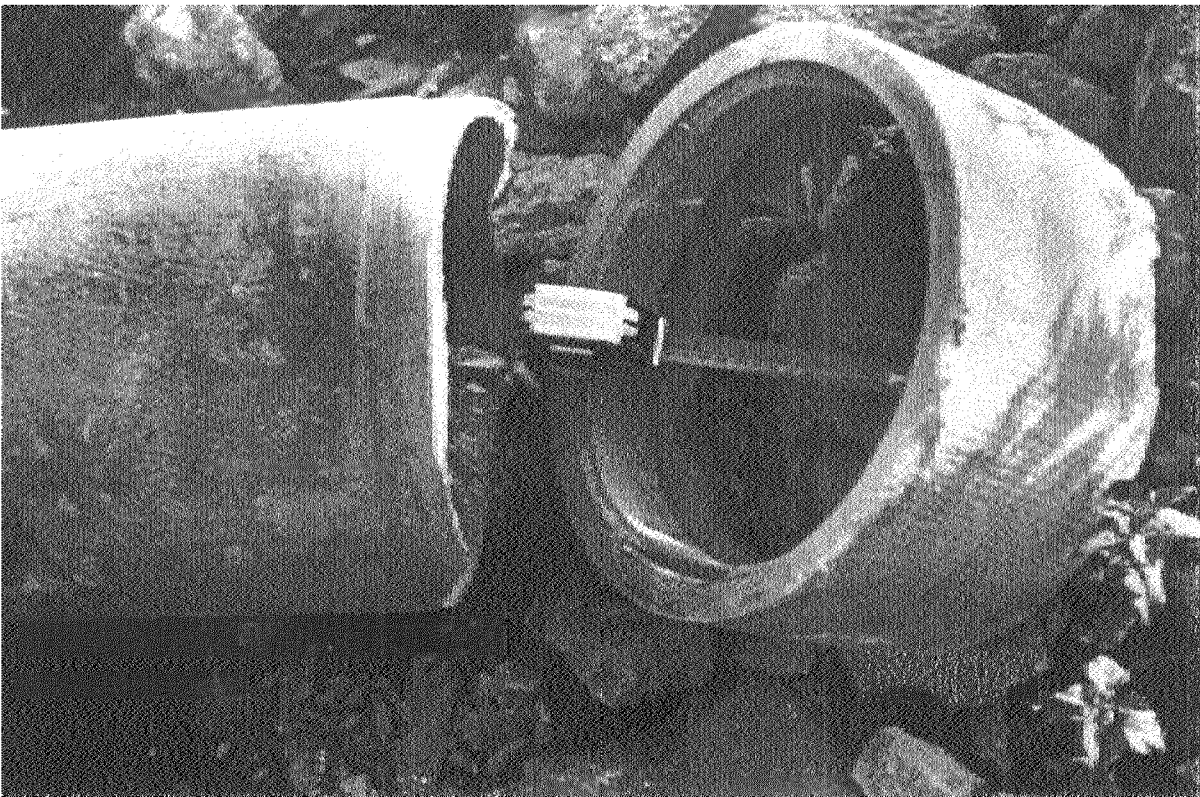
FIGURE 6-17 Break Near Joint Of An Asbestos Cement Pipe, 1985 Michoacan Earthquake
