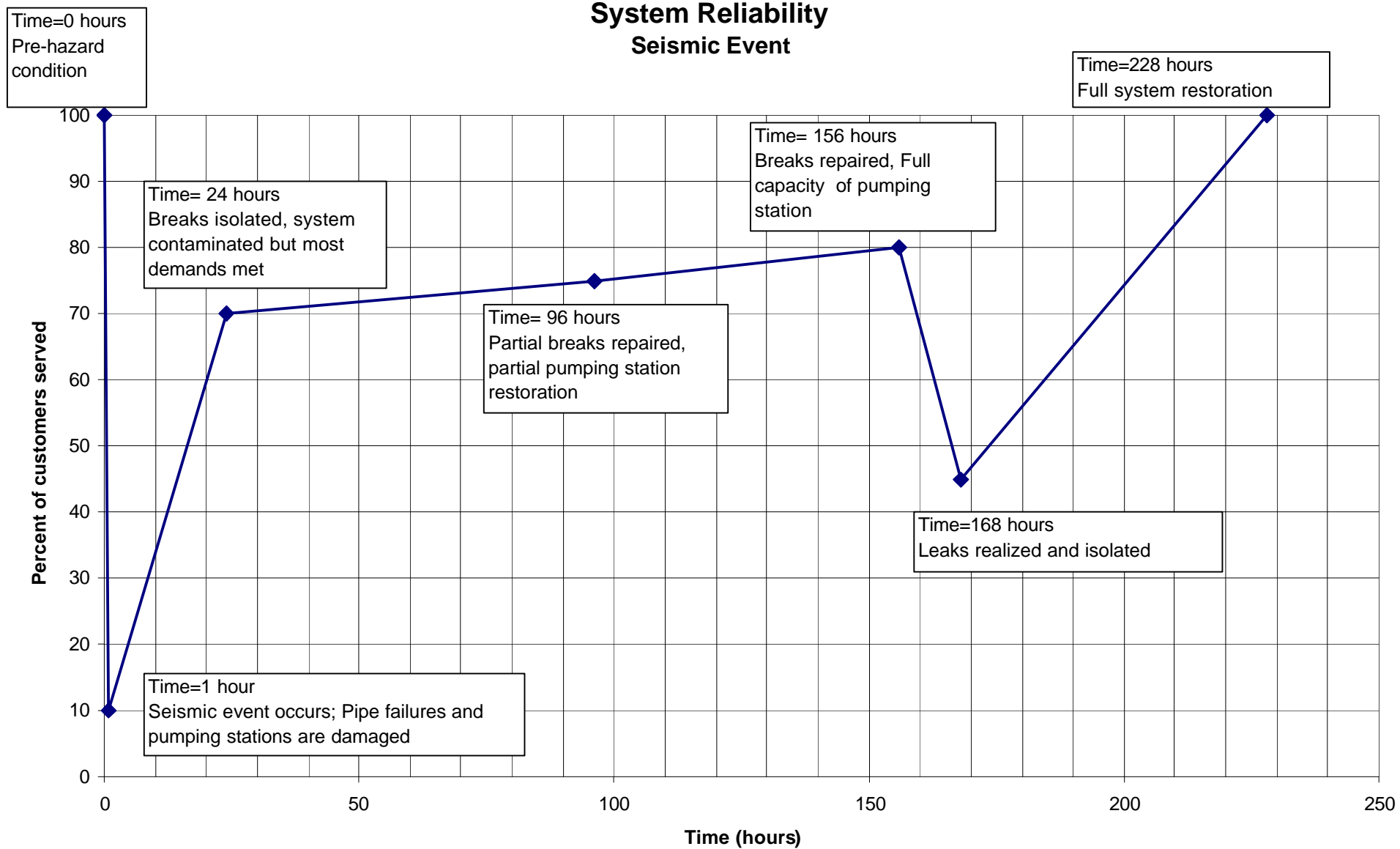
Figure 38: Hypothetical Earthquake System Reliability
