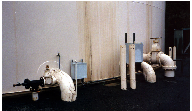
8 Rigid Piping to Tank (Photo courtesy Moulton Niguel Water District)
