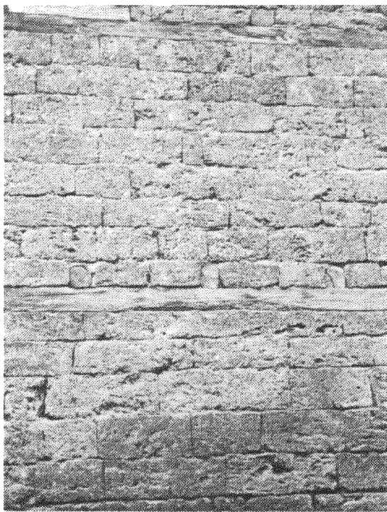
Stone masonry with timber reinforcement (22)
