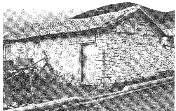
Poor stone masonry in rural structure near Xanthi
