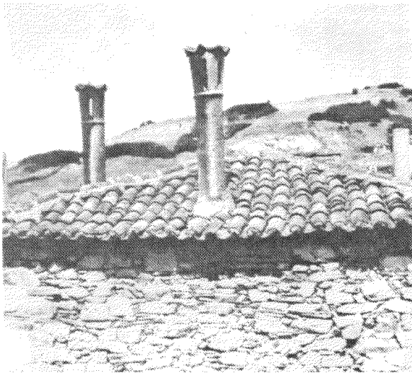
Stone masonry and chimneys in typical dwelling in Xalkidiki(23)
