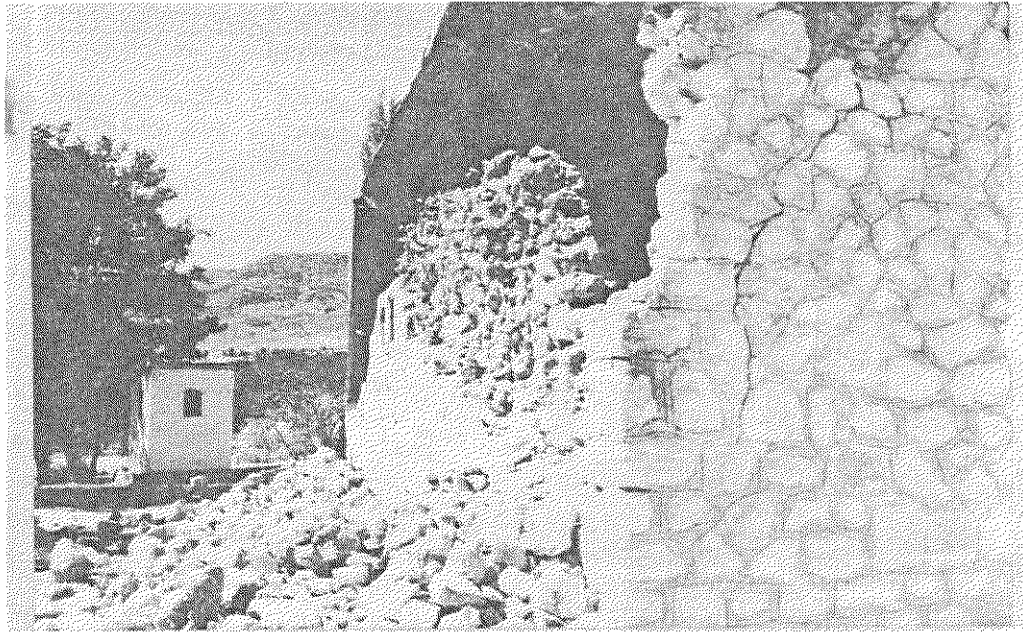
FIG. 3 INADEQUATE BOND BETWEEN TWO STONE LAYERS (Sept. 6, 1975, Lice Earthquake, Turkey)
