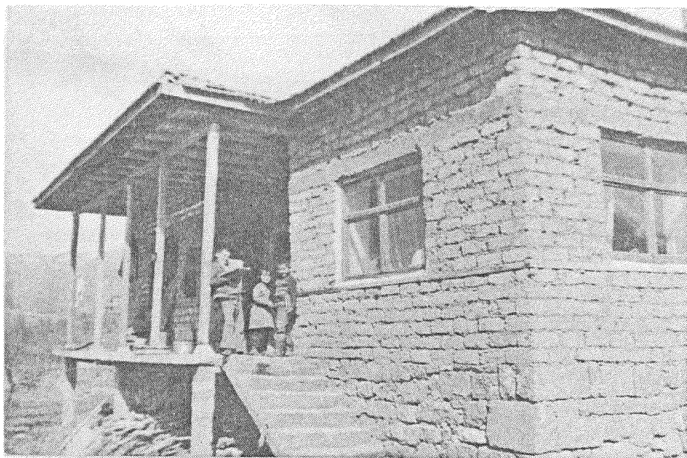
FIG. 2 A WELL - BUILT ADOBE HOUSE (Erzincan , Üzümlü town , Feb. 1978 , Turkey)
