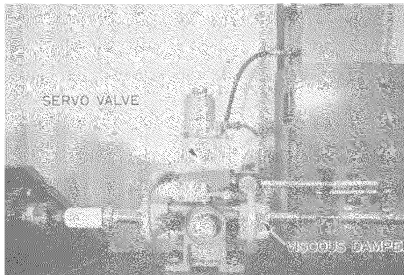
Photo 8 Variable Damper
