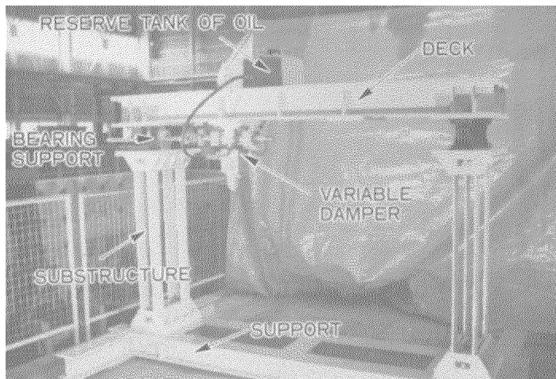
Photo 7 Bridge Model with Variable Damper
