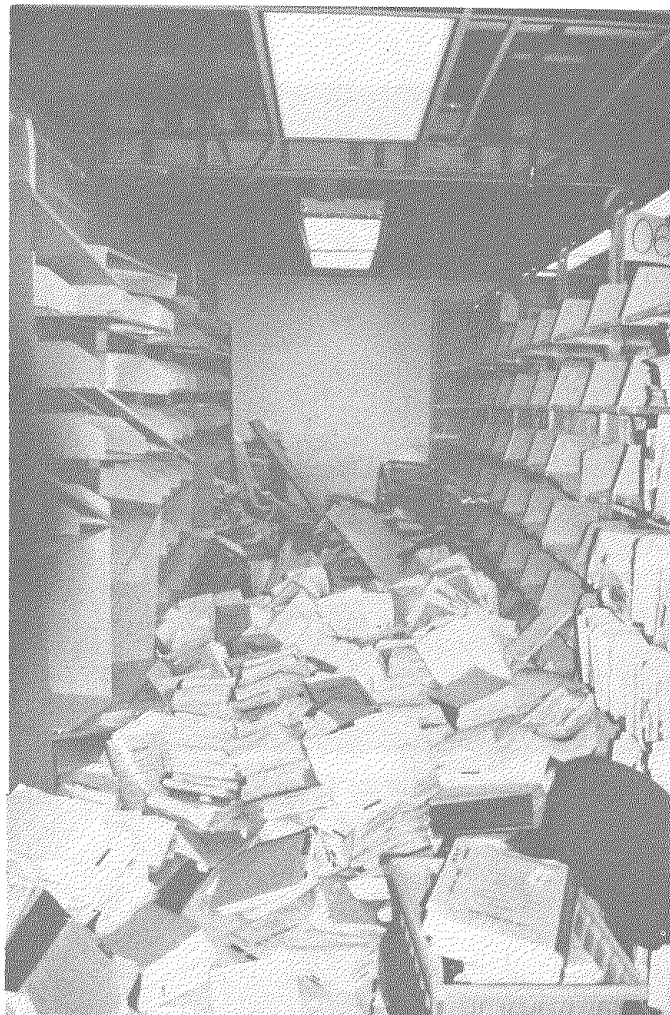
Fig. 35 Overturning of files at basement and nonstructural damage of gypsum boards in roof.
