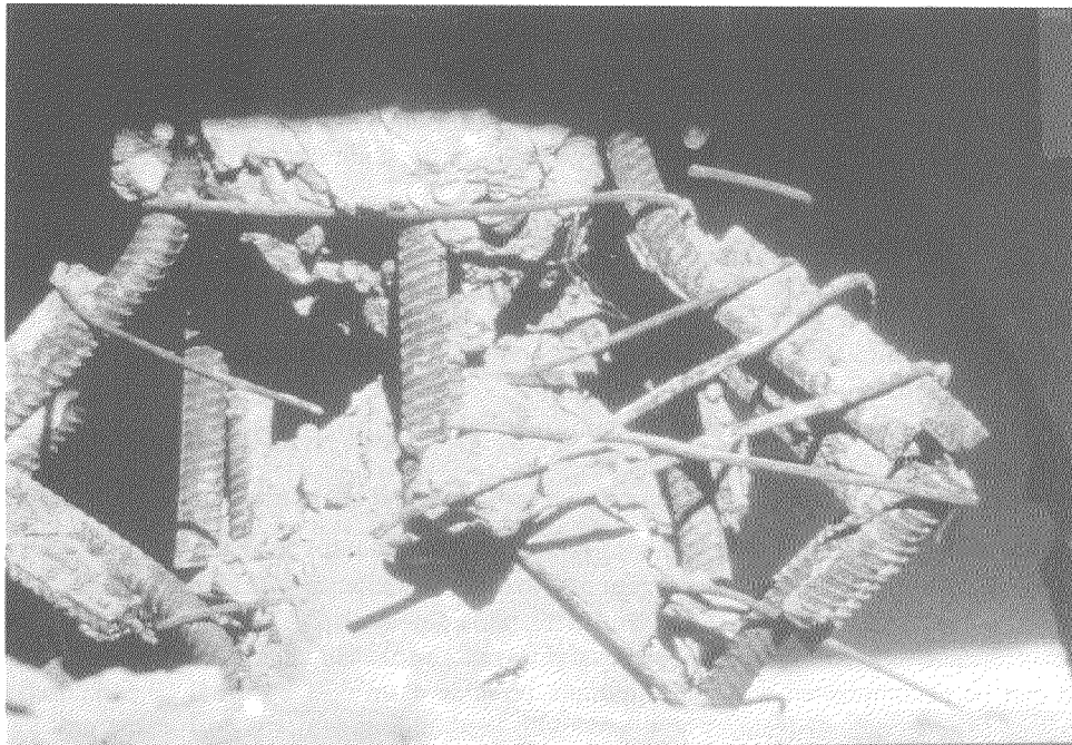
Fig. 6 (b) Failure of column-splice due to poor detailing and workmanship of ties and welding of main bars
