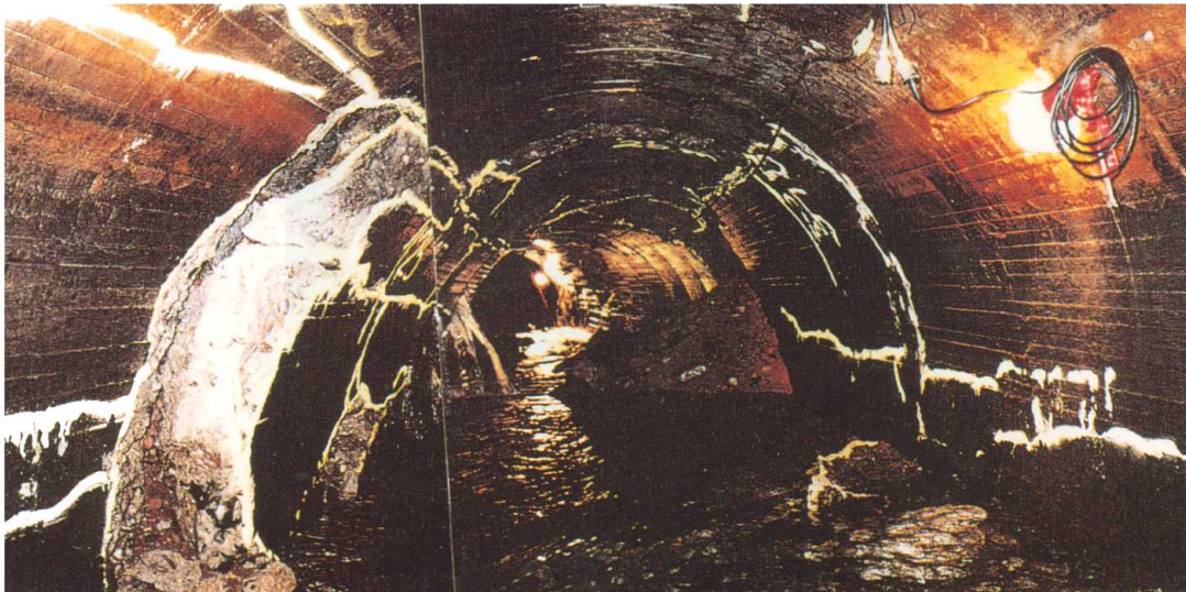
Photo 4 Damage to outlet tunnel (provided by Tohoku Electric Power Company)
