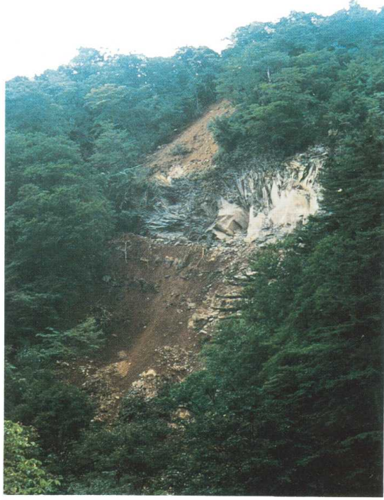
Photo 7 Basalt rock layer sandwiched in between loamy soils
