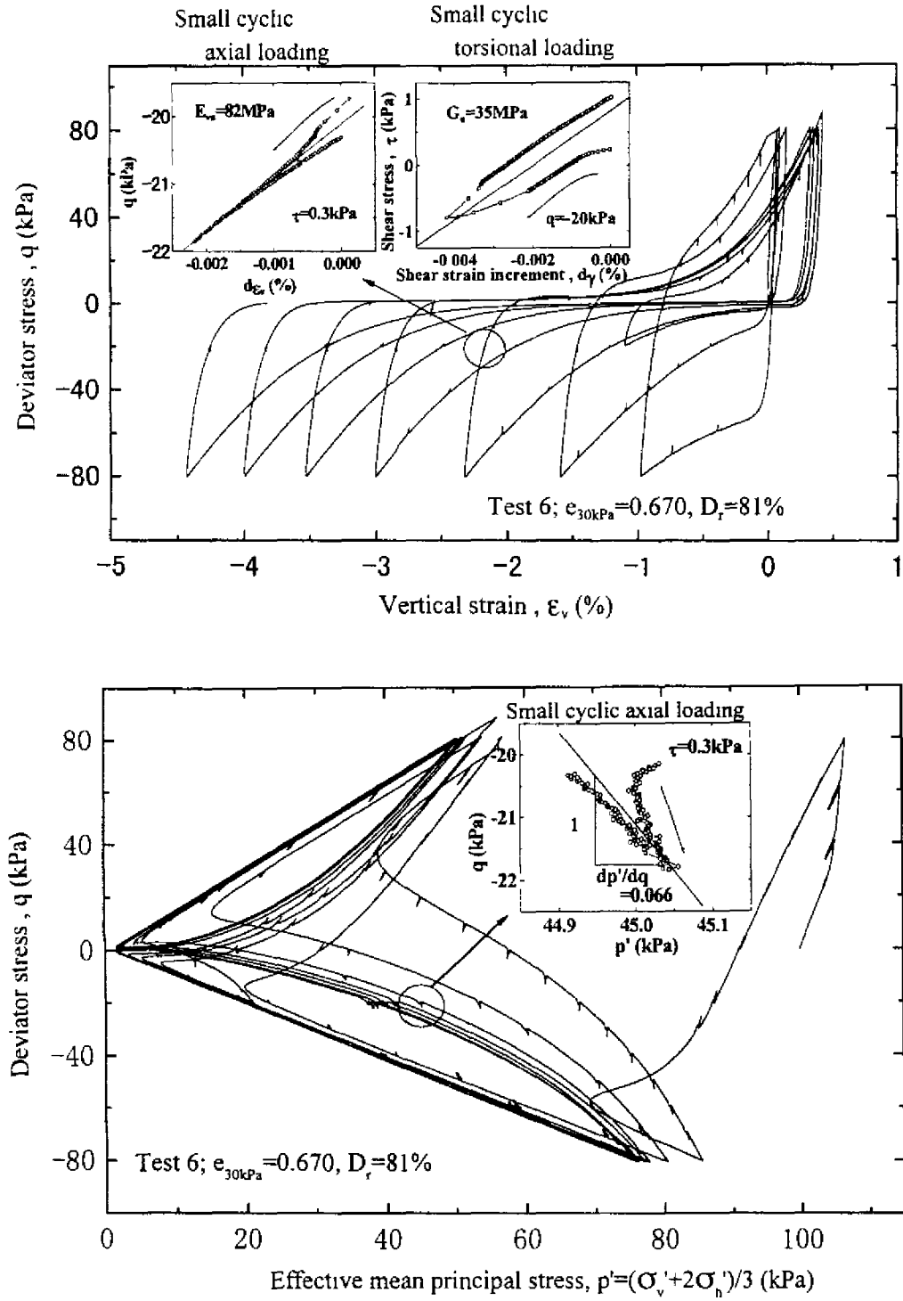
Figure 7 Results of test 6 during large amplitude undrained cyclic triaxial shearing, a) stress-strain relationship; and b) effective stress path
