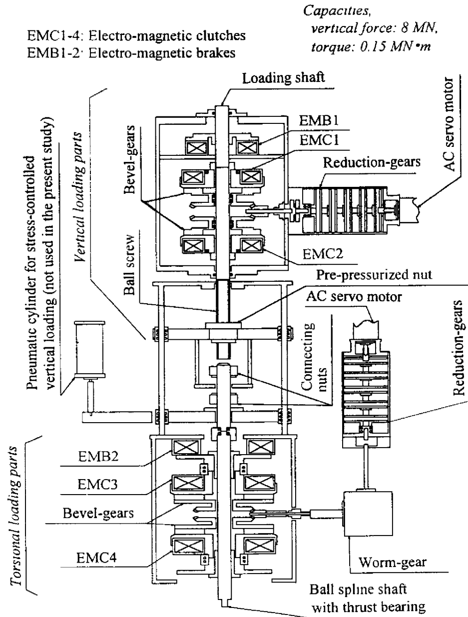
Figure 2 Torsional and vertical loading device
