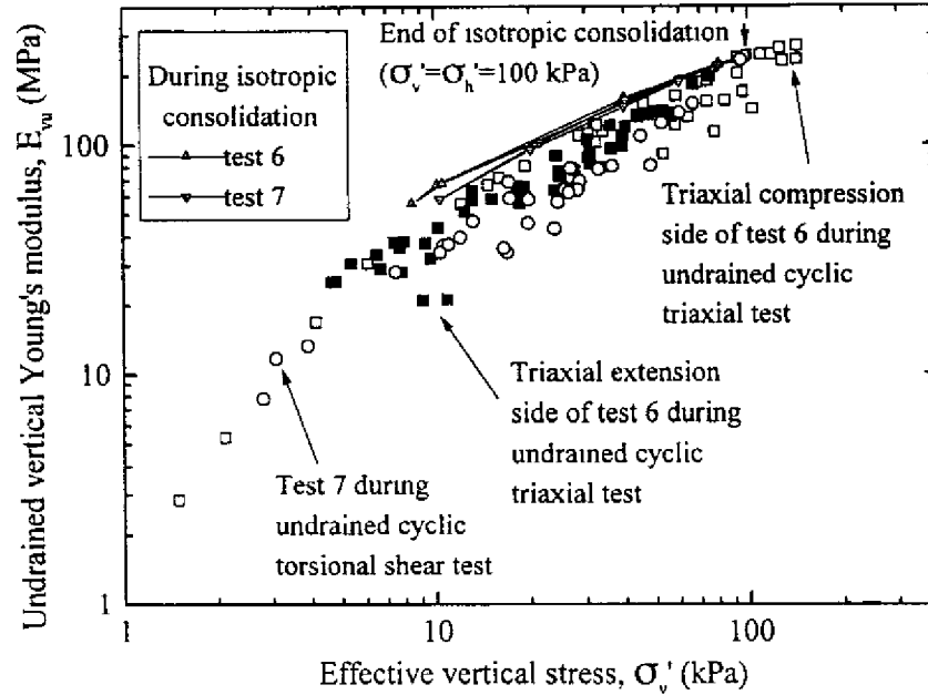
Figure 11. Undrained Young's modulus versus effective vertical stress
