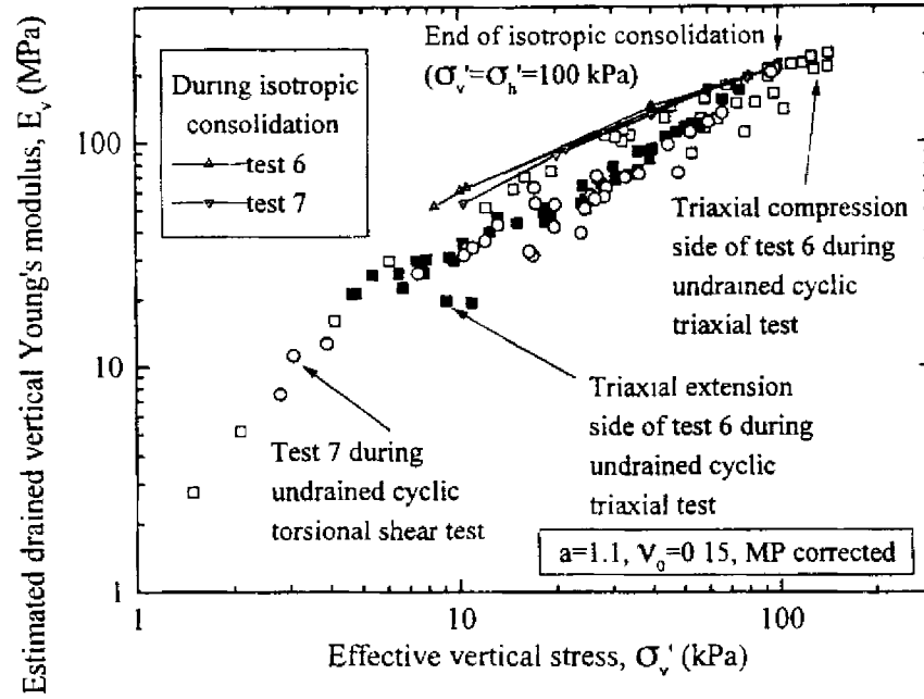
Figure 12 Estimated drained Young's modulus versus effective vertical stress
