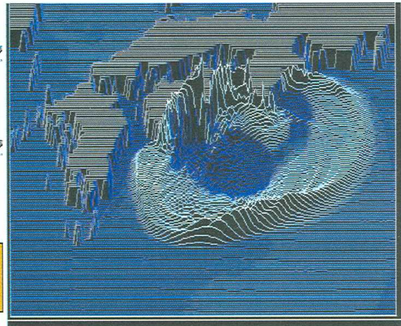
The propagation of tsunami (by computer simulation)
