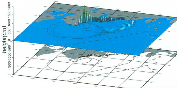
The propagation of tsunami (by computer simulation)
