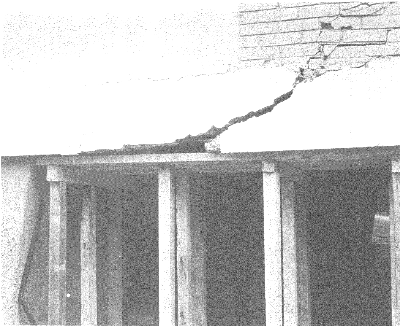
FIGURE 70.—Severe damage to flat beams and slab in the five-story reinforced-concrete Edificio ELGIN, in Guatemala City (Zone 14).
