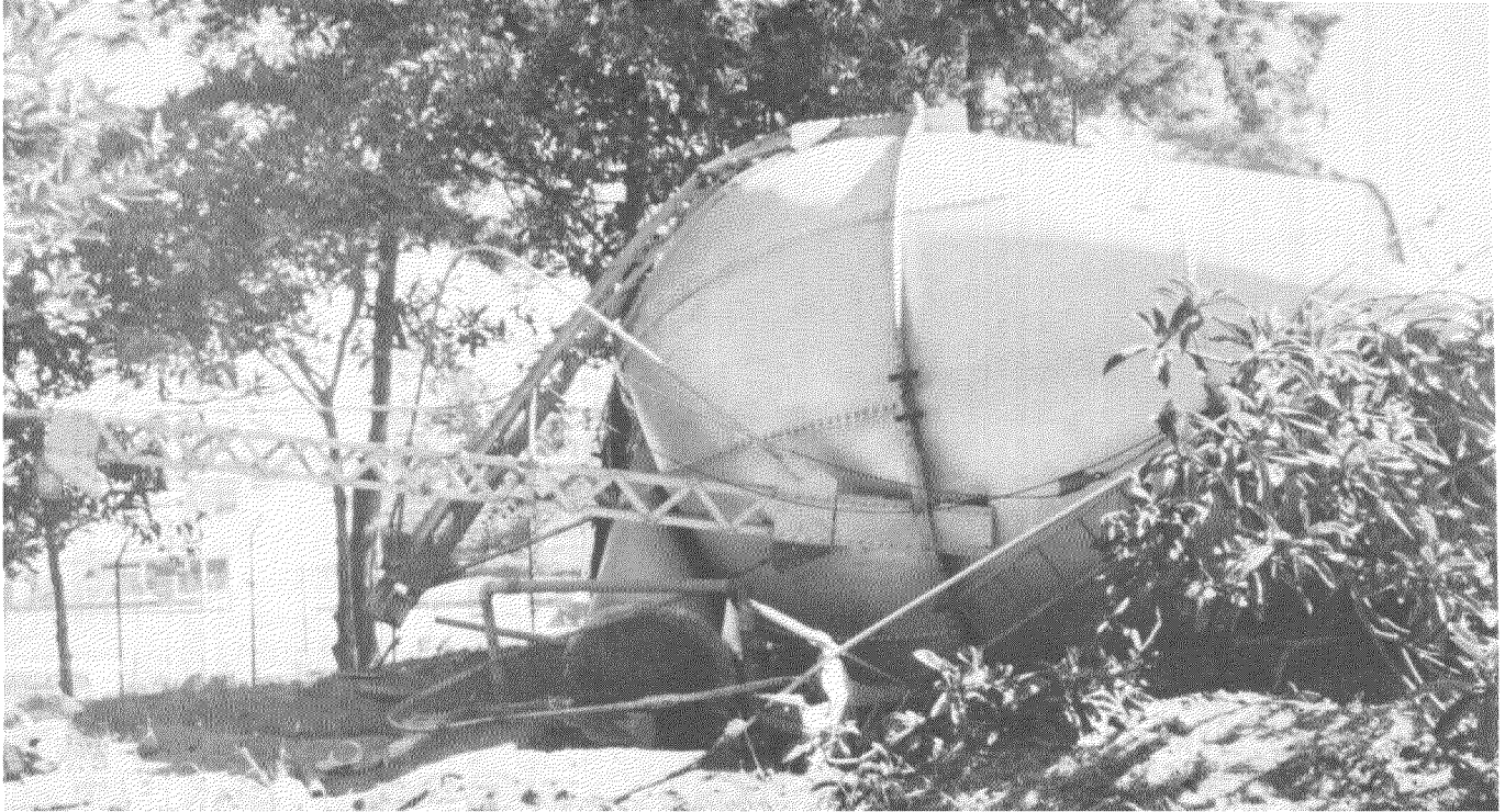
FIGURE 57.—Collapse of an elevated steel water tank in the Instituto Técnico Vocacional in Guatemala City (Zone 13).
