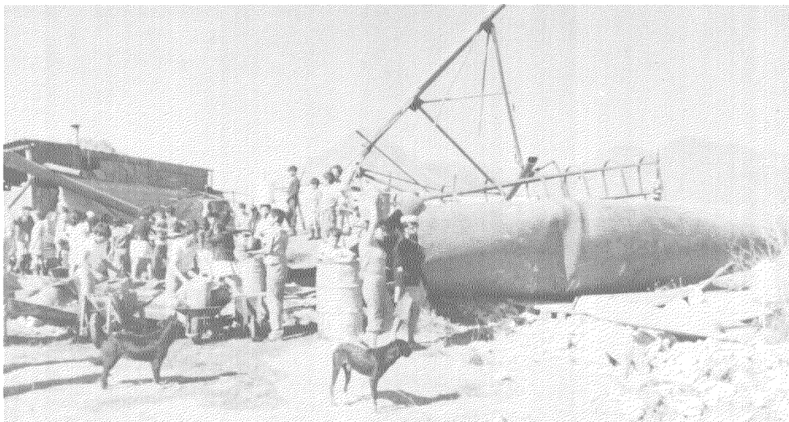
FIGURE 59.—Collapse of an elevated steel water tank in Villanueva, Colonia de los Planes, 22 km south of Guatemala City.
