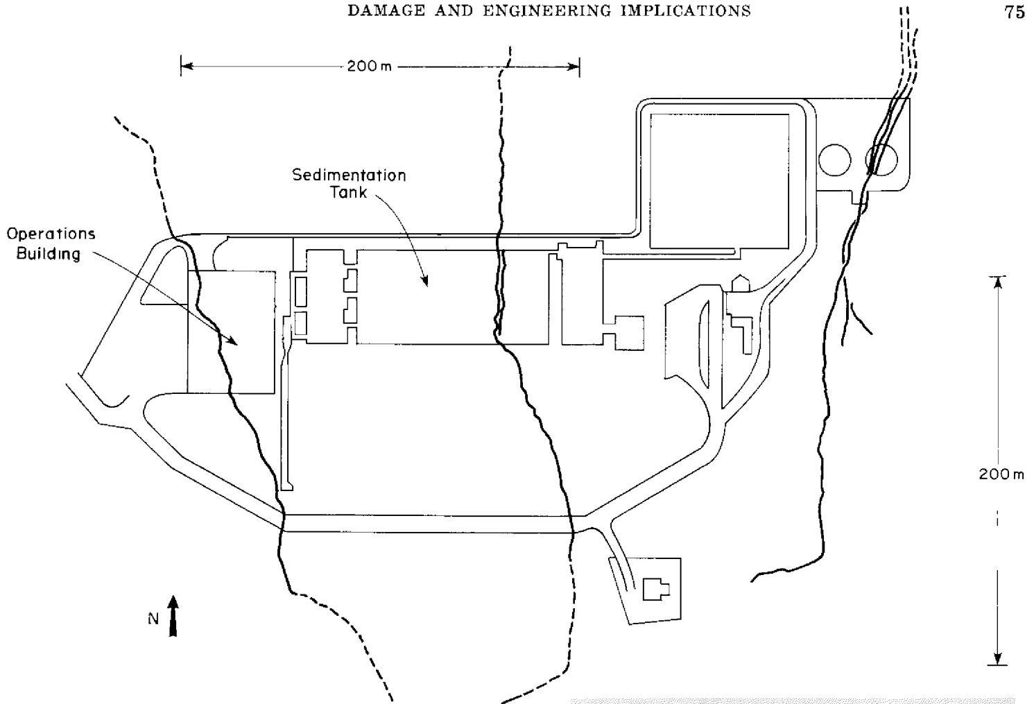
FIGURE 61.—Plan of sedimentation tank and Plant Lo de Coy of the XAYA-PIXCAYA project and cracks (heavy lines) running under and across the sedimentation tank.
