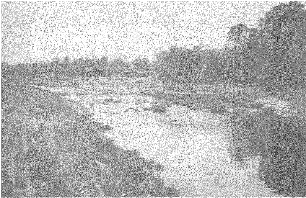
Fig. 18 Example of Natural Multifaceted Riparian Works
