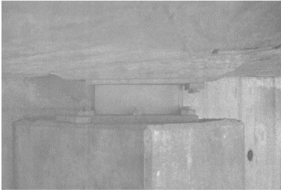
Fig. 5.7 Rocker bearing resting between sole plate above and masonry plate below, with missing keeper plate at top left (eastern end of bearing).
