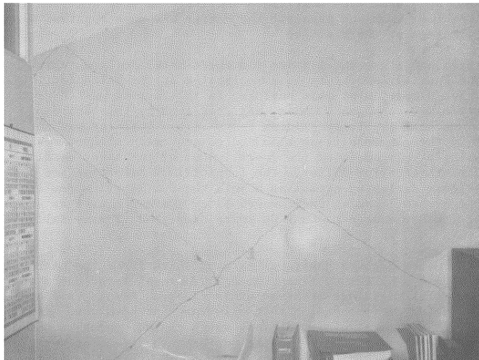
Fig. 7.40 Pattern of X cracks in shear wall at west end in first story of Administration Building, Delco Electronics facilities.
