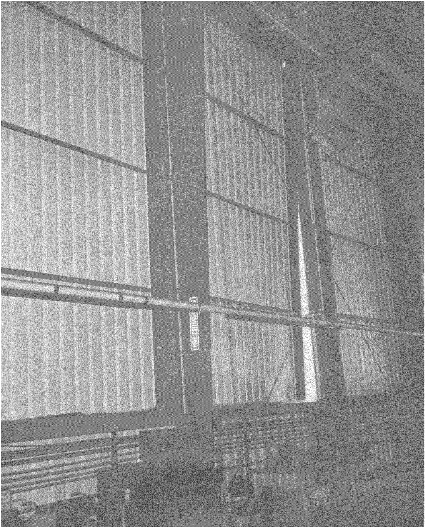
Fig. 7.47 Explosion panel which broke loose at the corner during the earthquake, Flight Physics Laboratory, Delco Electronics facilities.
