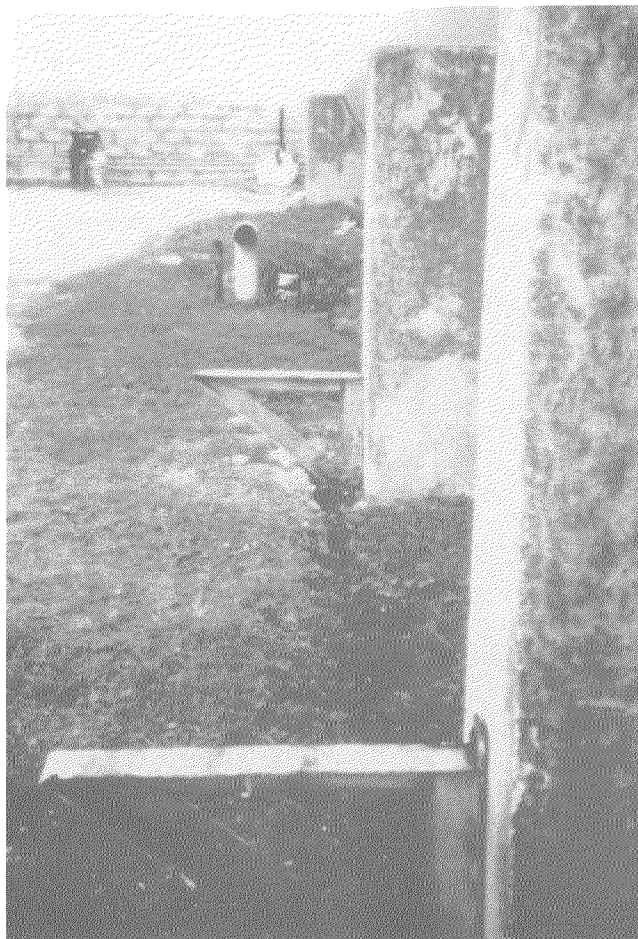
Figure 9: Uniform settlement and lateral movement of the oil tanks. Shell Oil Terminal
