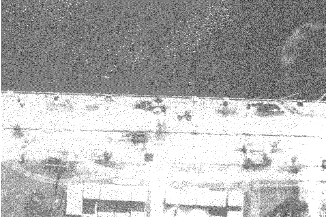
Figure 14 Aerial view showing concentration of lateral movement and settlement behind the bulkhead, U S. Navy port facilities
