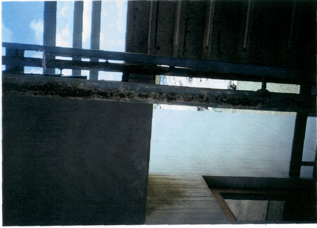
PHOTO 16 Corrosion spots along the steel column in the emergency stairway
