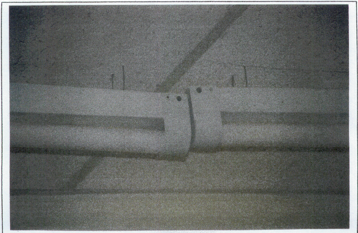
Photo 12 - Suspended light fixtures in the Hospital Inadequately attached, even without an earthquake
