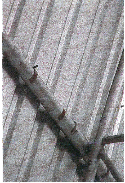
Photo 16. The hooked bolt detail used in both the Boiler House and the Laundry House to tie the roof sheets to the purlins. This detail is inadequate for hurricane resistance.
