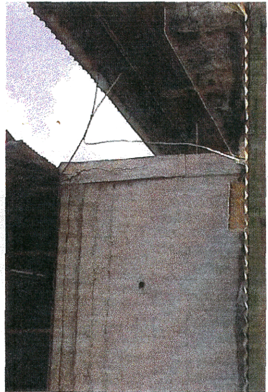
Photo 14. A long vertical crack in the Southern corner column of the Boiler House.
