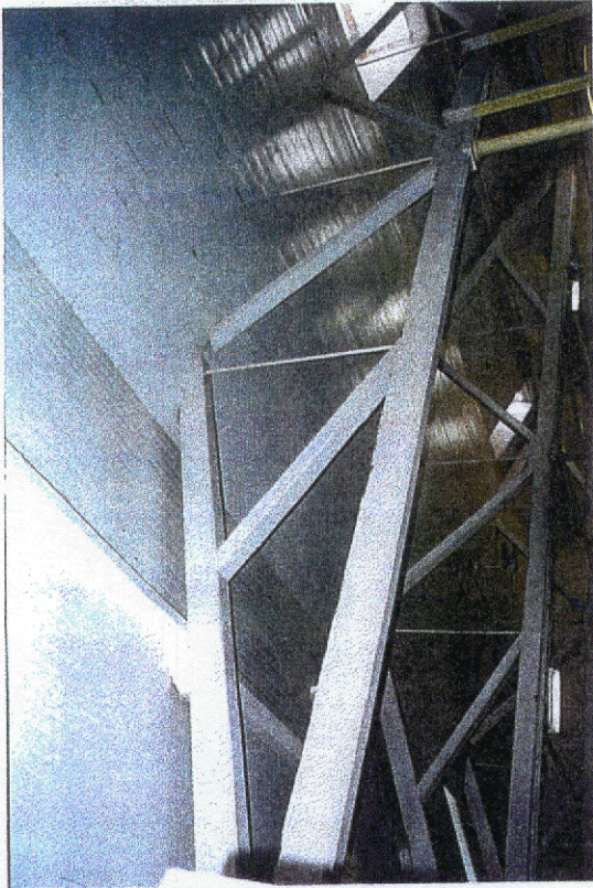
Photo 25: Typical roof truss in Femal Ward.
