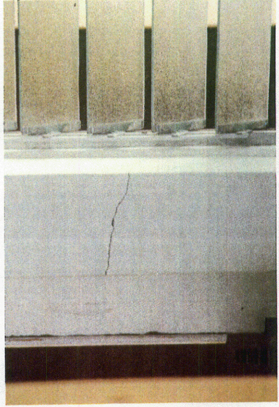
Plate 12 Cracked Masonry Pier (after removal of wall)
