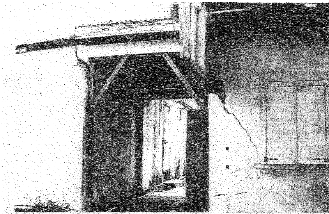
Photo HL-3: Cracks at corner of Boiler Room.
