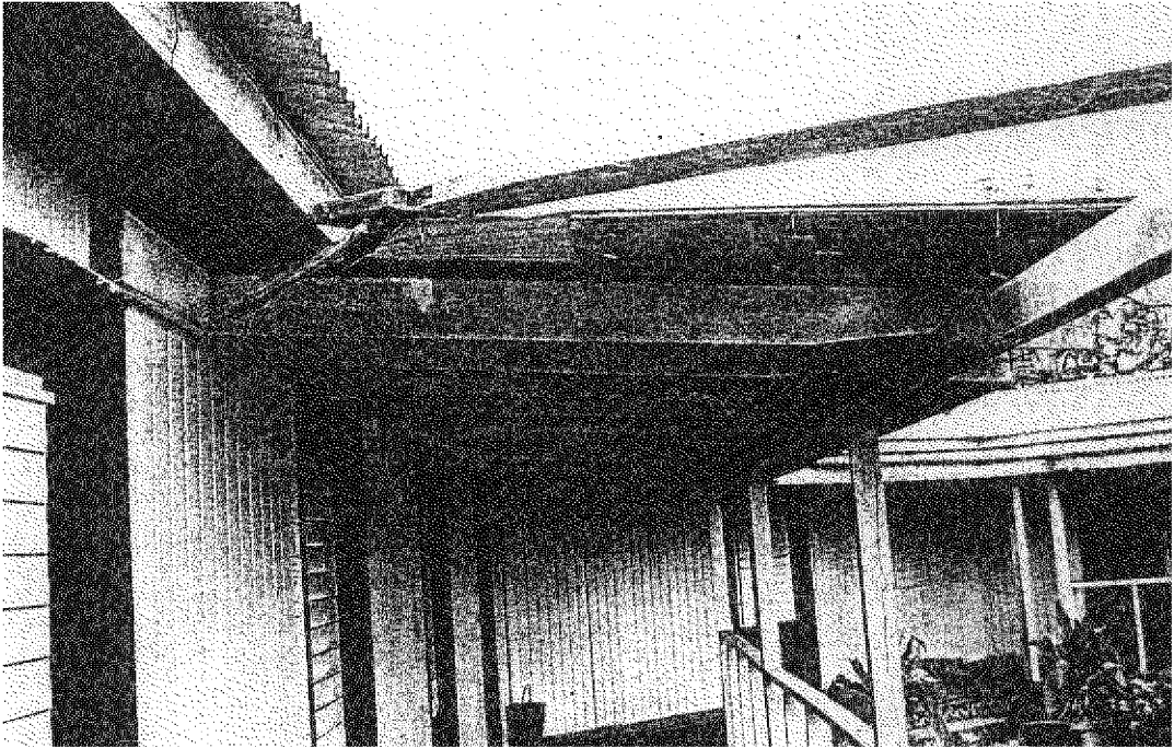
Photo M-1: Verandah roof blown off.
