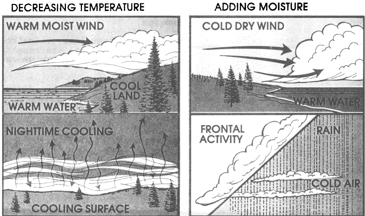
FIGURE 13 -- CLOUD DEVELOPMENT PROCESSES
