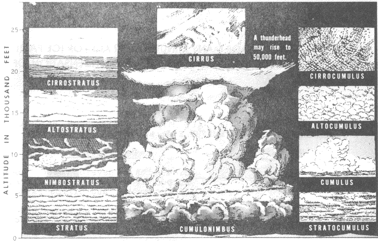
FIGURE 12 -- KINDS OF CLOUDS IN THE ATMOSPHERE
