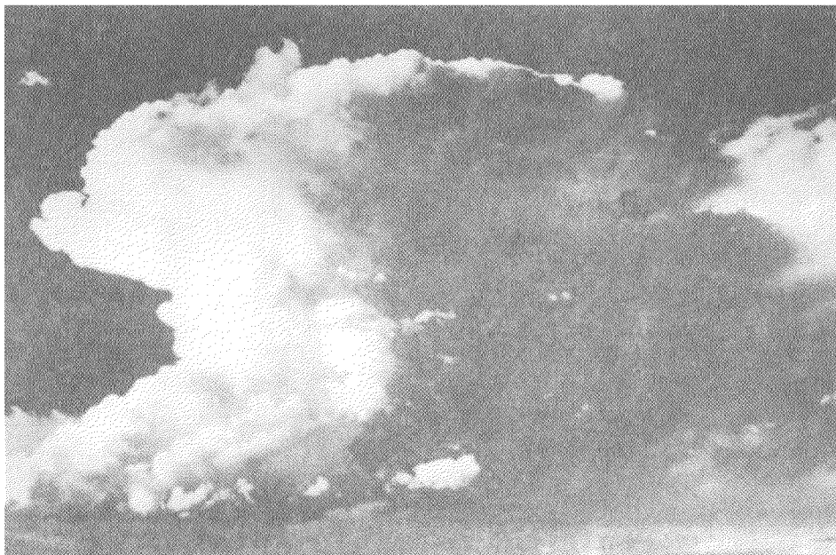
FIGURE 15 — CUMULONIMBUS CLOUDS OR THUNDERHEADS
