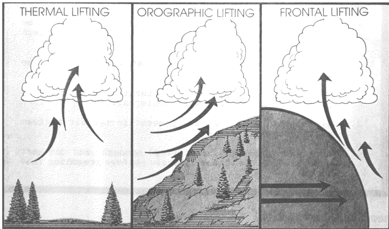
FIGURE 14 — LIFTING PROCESSES IN THE ATMOSPHERE
