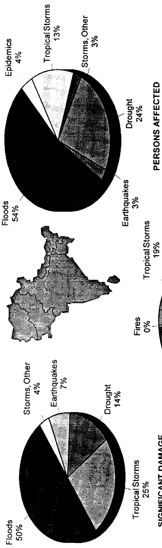
% of Significant Disasters by Type and Category
