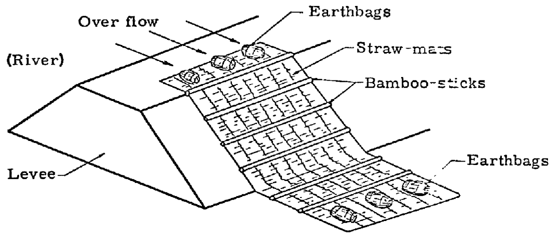
Fig. 3.19 Diagram of straw-mat protection to levee
