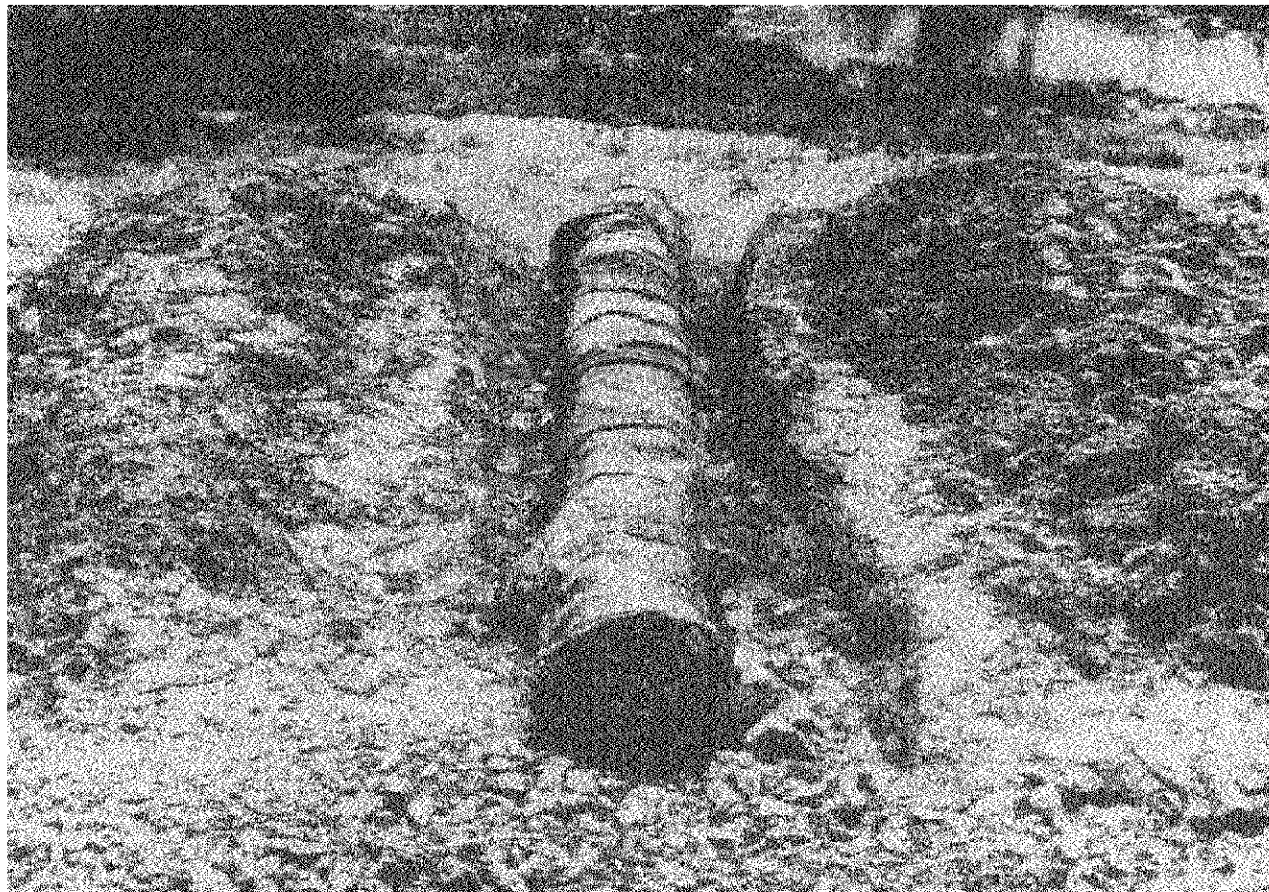
FIG. 3.23 - The construction of a willow-cylinder filter.
