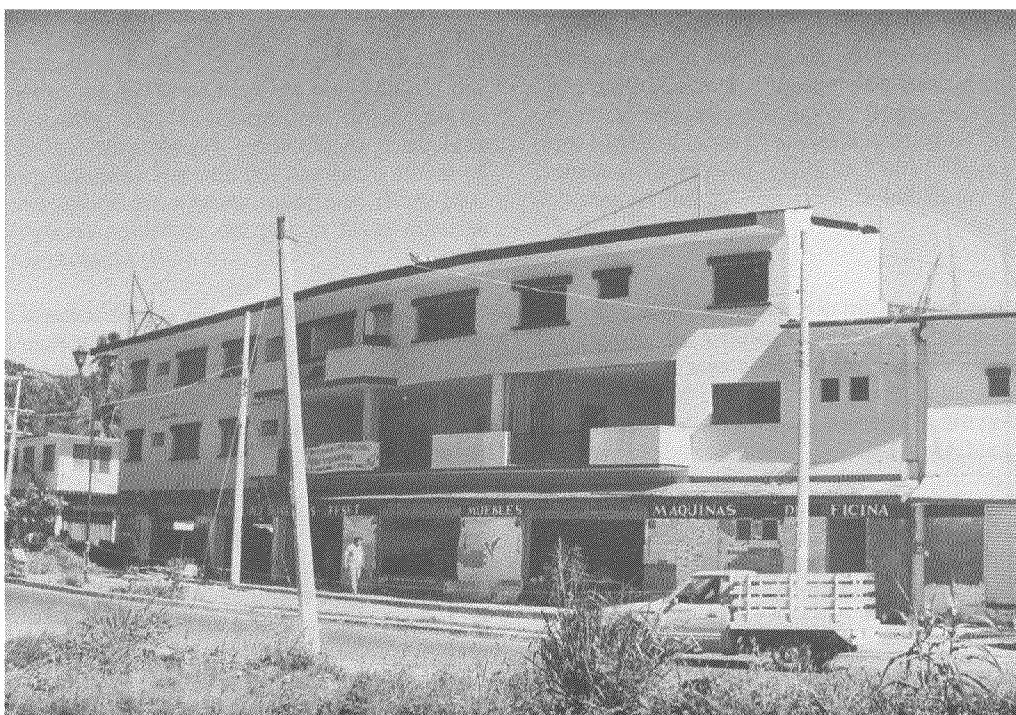
Photo 59.- West part of Impresos López after the 1985 earthquakes [1].
