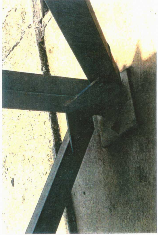
Photo 29: Radiator support fixing detail, Power Station
