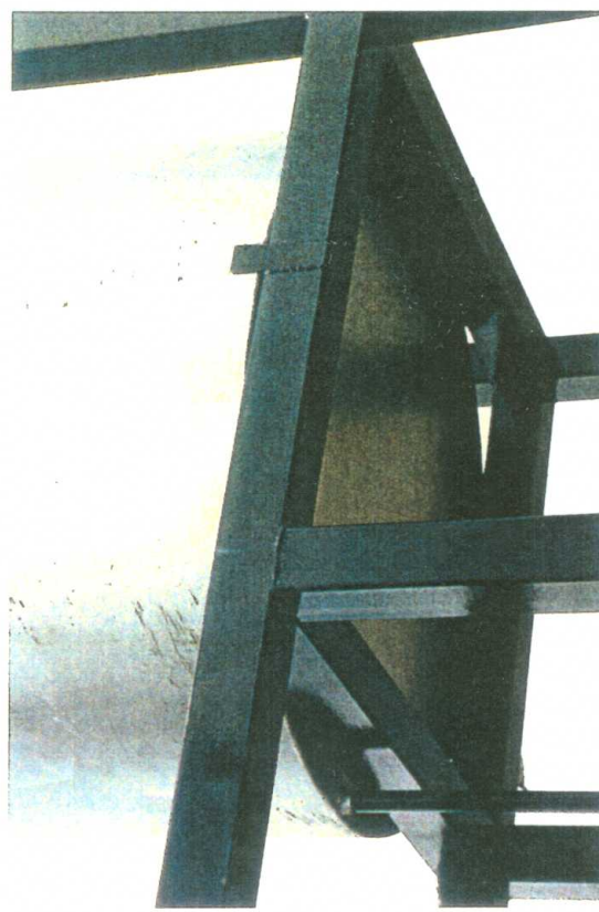
Photo 35: Typical stack support, Peak Lopping Station
