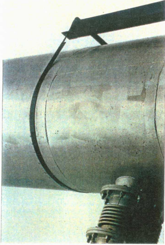
Photo 36: Typical stack support and connection to engine, Peak Lopping Station
