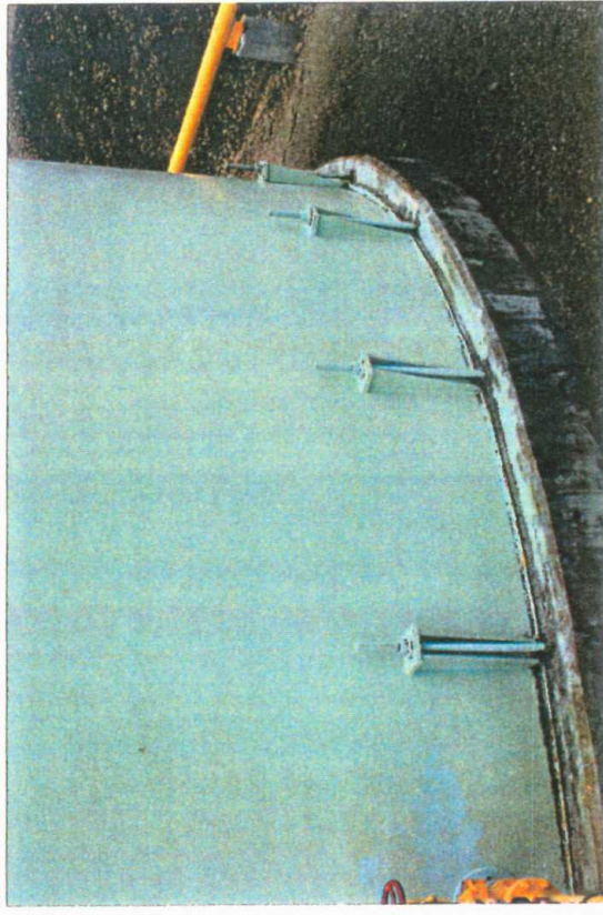
Photo 53: Base fixing detail, large Fuel Tanks
