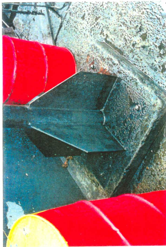
Photo 66: Base detail, Exhaust Stacks support
