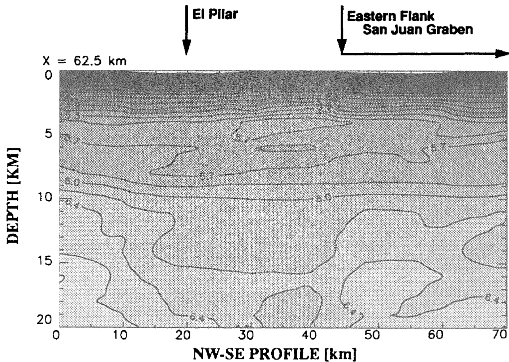
Figure 9: Cross-section at X=62.5 km. Vertical arrow is indicating the surface expression of the El Pilar Fault and the horizontal the one of the San Juan Graben. (For more explanations see text).
