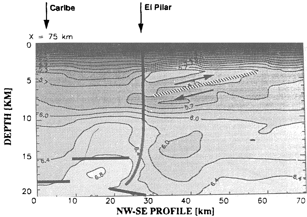
Figure 10: Cross-section at X=75 km. Arrows are indicating the surface expression of the El Pilar and North Coast faults. (For more explanations see text).
