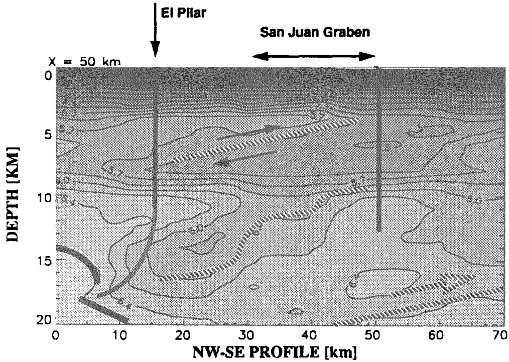
Figure 8: Cross-section at X=50 km. Vertical arrow is indicating the surface expression of the El Pilar Fault and the horizontal the one of the San Juan Graben. (For more explanations see text).
