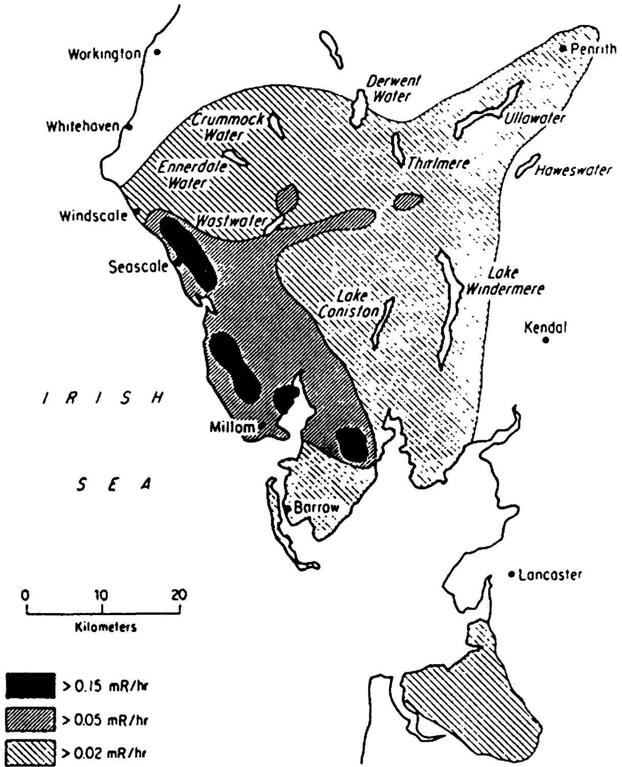
Figure 4. Environmental \gamma -radiation levels near Windscale five days after fire. 2
