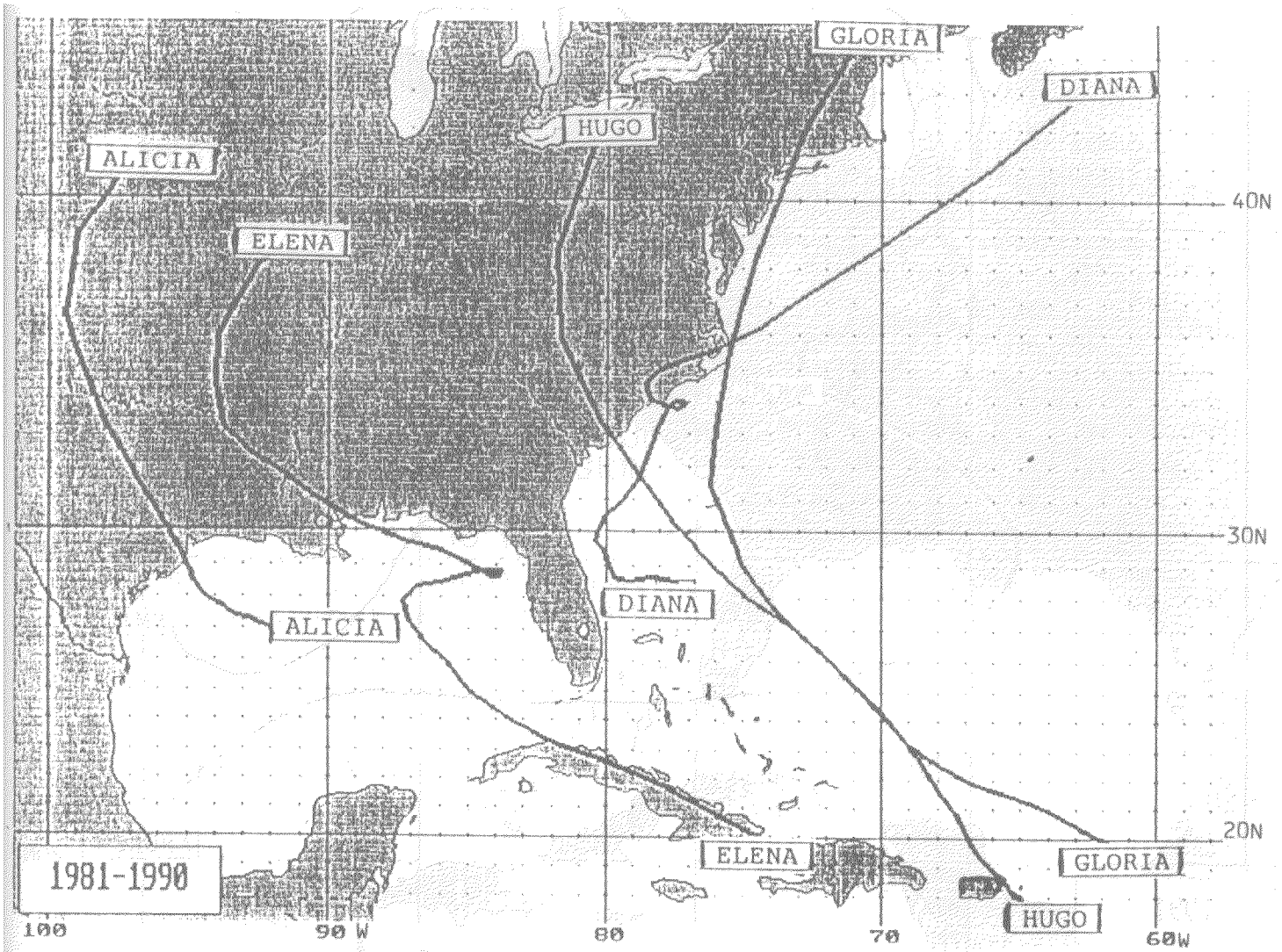
Fig. 4 (e). Major hurricanes striking continental United States. 1981 through 1990.
