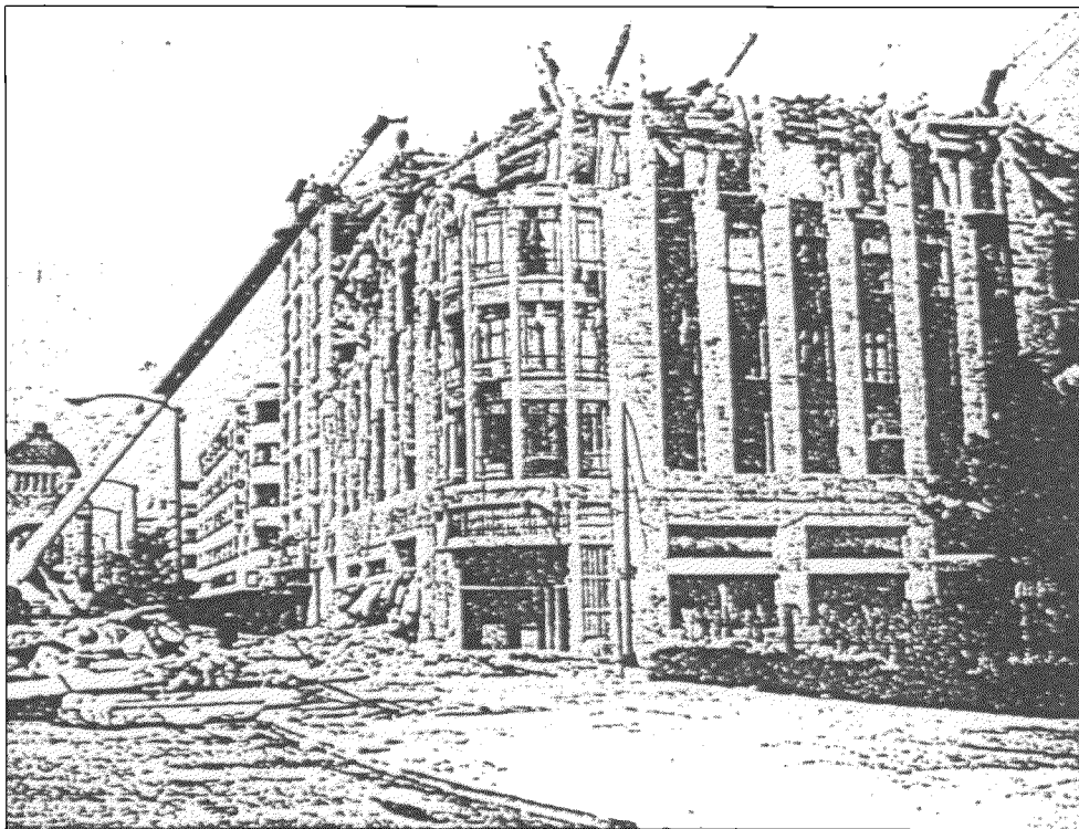
Older concrete building -- upper floor collapse
