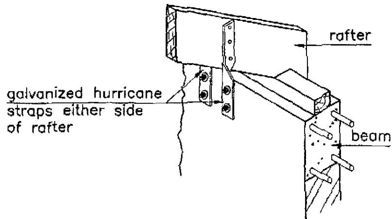
Timber rafter connection to concrete
