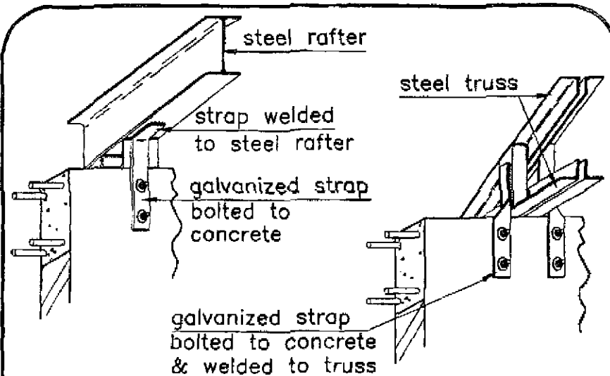
(after welding, apply rust-proofing coating) Steel truss and rafter connection to concrete
