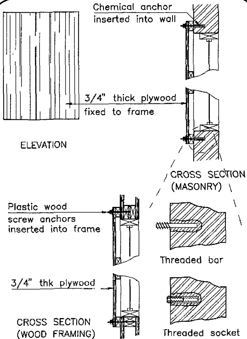
Pre-fabricated removable shutter Guide Ref. #10
