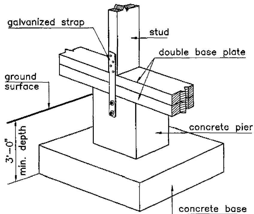
Stud to foundation connection Foundation anchorage
