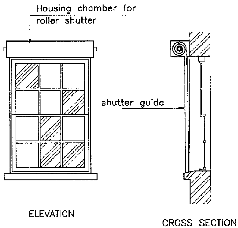
Roller shutter
